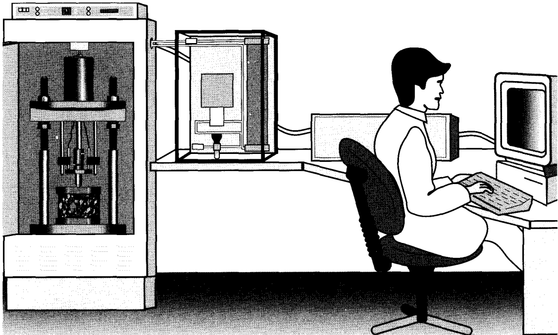
FIGURE 4. SCHEMATIC OF NOTTINGHAM ASPHALT TESTER. (The Nottingham Asphalt Tester (NAT) is used to measure the mechanical properties of asphalt concrete such as elastic stiffness (resilient modulus) and resistance to permanent deformation [15].)
