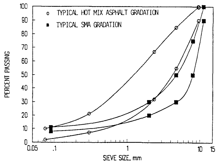
FIGURE 2. COMPARISON OF TYPICAL DENSE GRADED HOT-MIX ASPHALT (HMA) AND STONE MASTIC ASPHALT (SMA) GRADING BANDS. (Coarse aggregate (plus 2 mm) about 70 to 80 percent, fine aggregate (2 mm to 90 \mu\text{m} ) about 12 to 17 percent and filler (minus 90 \mu\text{m} ) about 8 to 13 percent for SMA. SMA coarse aggregate top size typically between 11 and 16 mm. Adapted from Report on the 1990 European Asphalt Study Tour (EAST) [6].)
