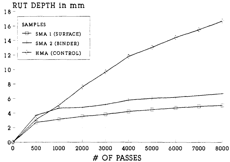
FIGURE 3. RUTTING TEST RESULTS FOR SMA 1 (SURFACE), SMA 2 (BINDER) AND HMA (HOT-MIX ASPHALT SURFACE) PAVEMENT SAMPLES.
