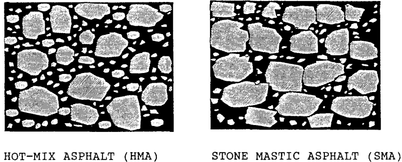
FIGURE 1. COMPARISON OF 'FLOATING' COARSE AGGREGATE IN HMA WITH STONE-TO-STONE 'SKELETON' IN SMA. (The point-to-point contact achieved in the SMA provide internal friction to resist load-induced shear. Adapted from Report on the 1990 European Asphalt Study Tour (EAST) [6].)
