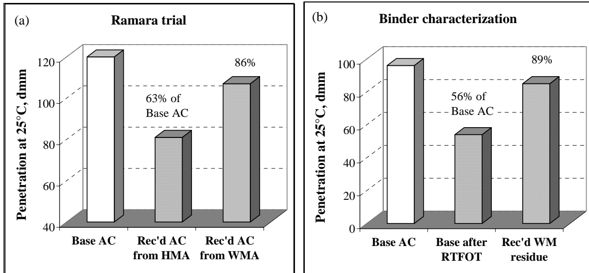
Figure 5. (a) Comparison of penetration of the base asphalt and recovered asphalt cement from Hot Mix Asphalt (HMA) and Evotherm® Warm Mix Asphalt (WMA) core samples taken during the Ramara Township trial (b) Data demonstrates that the residue recovery procedure developed here closely simulates the heat history of the mixing and paving process when using the Evotherm® warm mix emulsion system.
