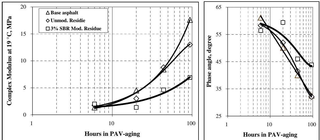
Figure 18. (a) Complex modulus and (b) phase angle of the base asphalt, unmodified Evotherm®, and 3% Styrene-Butadiene-Rubber (SBR) latex-modified Evotherm® binders as a function of PAV-aging. The SBR latex-modified Evotherm® residue shows only limited increase in G^* after 44 and 94 hour PAV-aging time. The phase angle of the 3.0% SBR latex-modified residue also remain above 45^\circ even up to 44 hours PAV-aging time.
