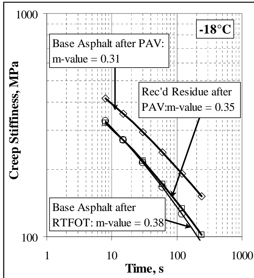
Figure 7. Measured creep stiffness of the base asphalt and unmodified Evotherm ® binder after PAV-aging at -18°C. The data for the base asphalt after RTFO-aging is also included for comparison.
