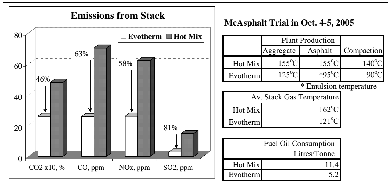
Figure 1. Summary of Evotherrm® and Hot Mix Plant Production at Ramara Township [10]
